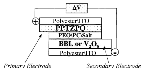
Figure 2. Electrochromic cell.
