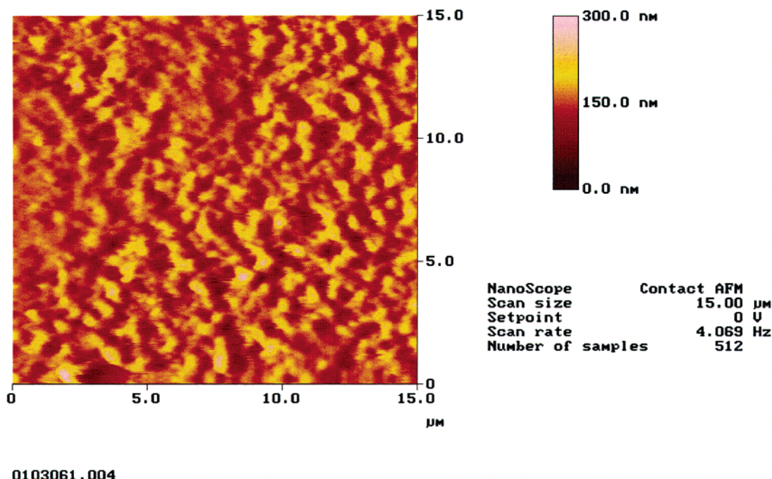
Figure 10. AFM image of PPTZPQ film spin-coated over an ITO electrode.
